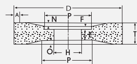
Type 25—Relieved & Recessed One Side, Relieved Other Side
