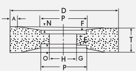
Type 26—Relieved & Recessed Both Side
