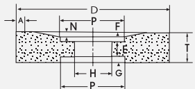
Type 24—Relieved & Recessed One Side, Recessed Other Side
